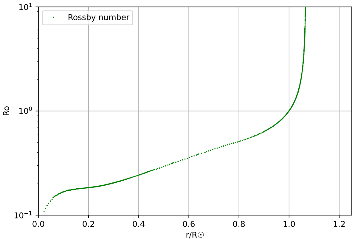
Rossby number, profile 156, age 6.62 \times 10^9
